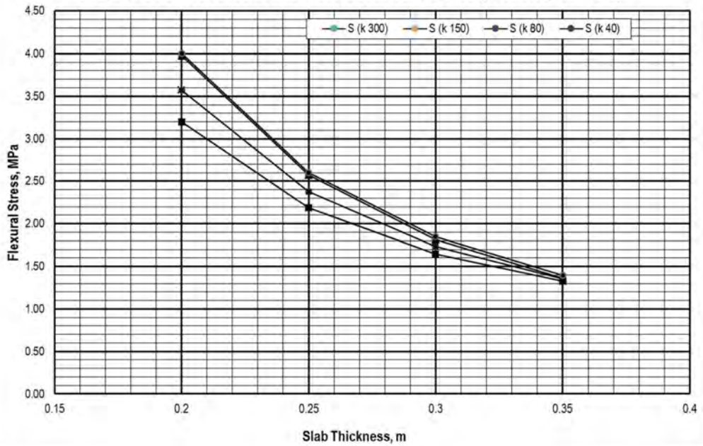
Stress Chart due to Tandem Axle: without Concrete Shoulder ( P=300 \text{ kN} , \Delta T=10^\circ\text{C} )
