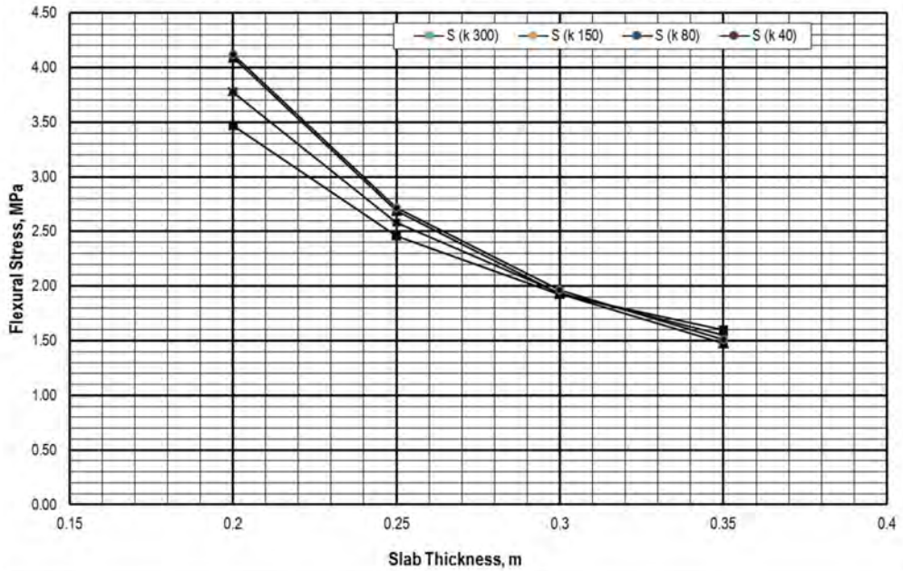
Stress Chart due to Tandem Axle: without Concrete Shoulder ( P=300 \text{ kN} , \Delta T= 15^\circ\text{C} )
