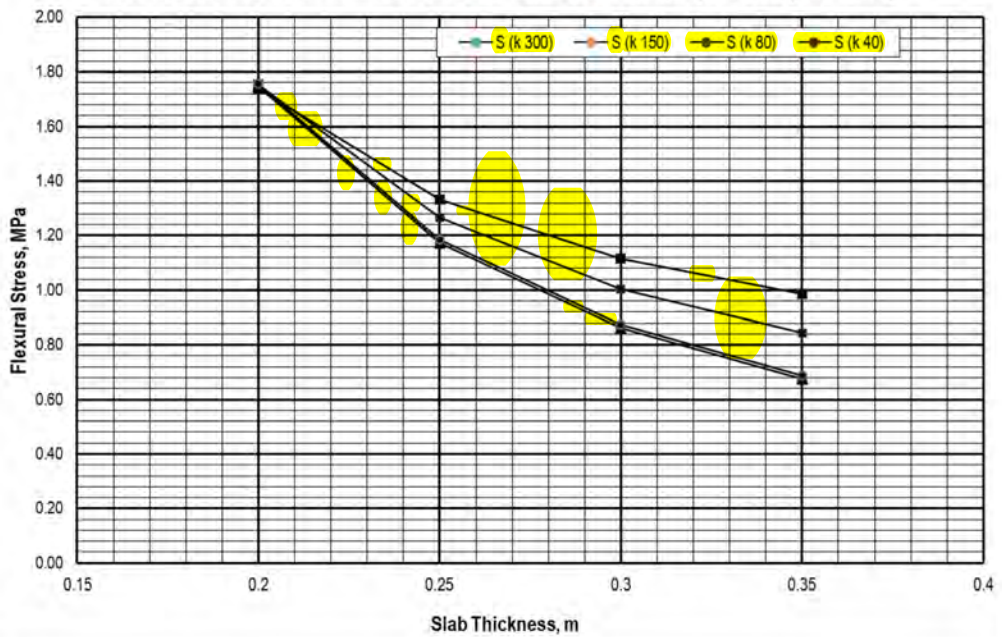
Stress Chart due to Tandem Axle Load with Concrete Shoulder ( P=160 \text{ kN} , \Delta T=15^\circ \text{ C} )
