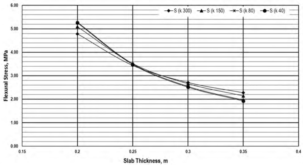
Stress Chart for Bottom-up Cracking Analysis Without Concrete Shoulders ( P=160\text{ kN} , \Delta T=20^\circ\text{C} )
