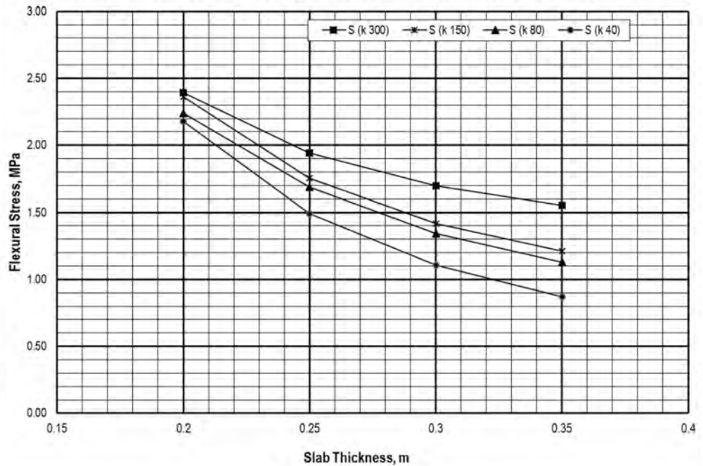
Stress Chart due to Single Axle Load with Concrete Shoulder ( P=80 \text{ kN} , \Delta T=20^\circ \text{ C} )
