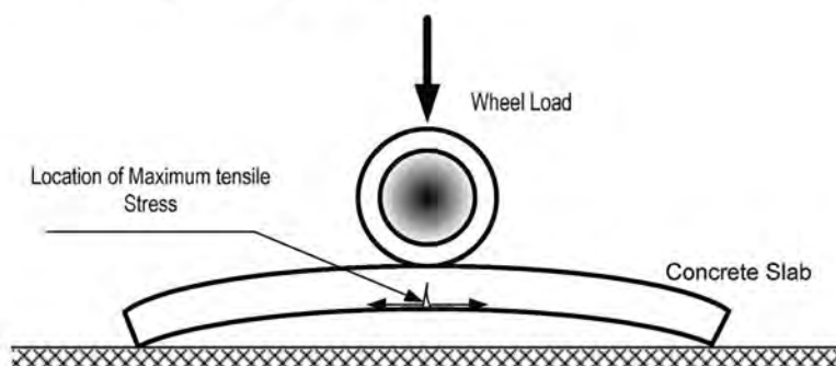
Figure 5 Axle Load Placed at the Middle of the Slab during Mid-day
