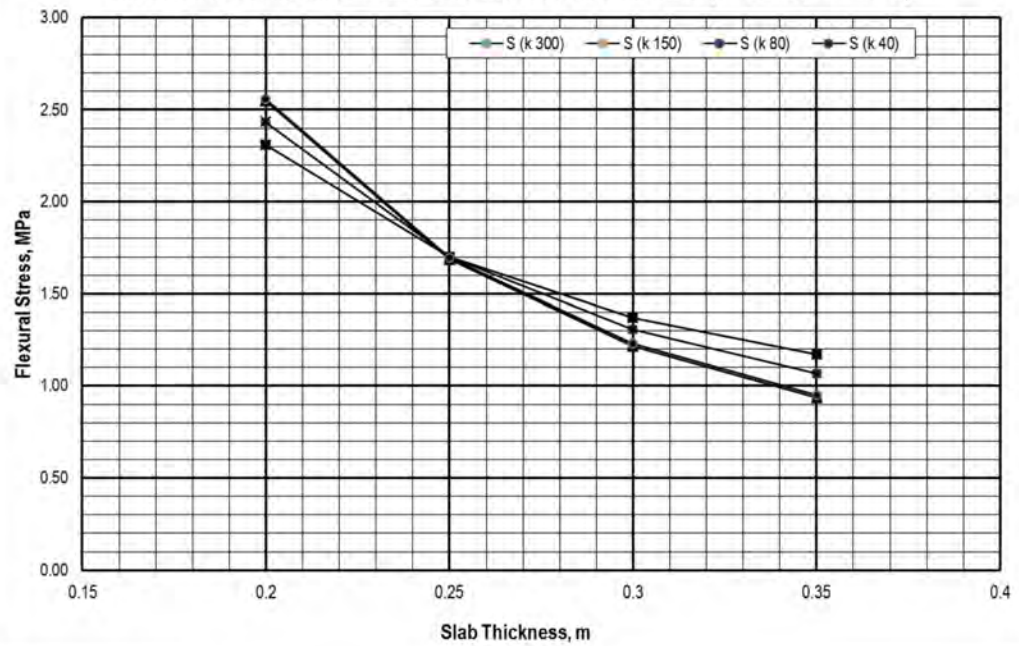
Stress Chart due to Tandem Axle Load with Concrete Shoulder ( P=240 kN, \Delta T=15^\circ C)
