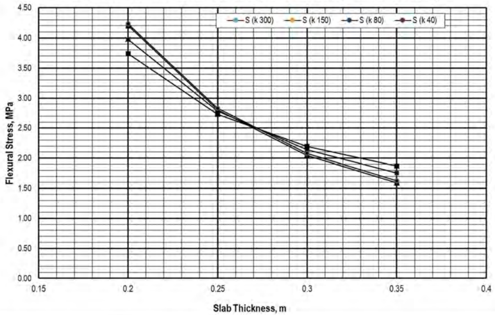
Stress Chart due to Tandem Axle: without Concrete Shoulder ( P=300 \text{ kN} , \Delta T=20^\circ\text{C} )
