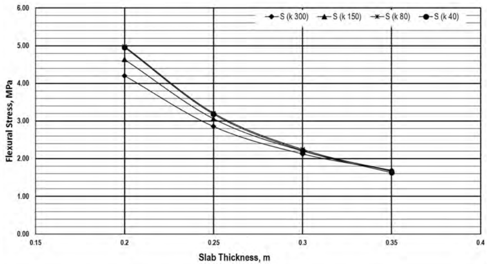
Stress Chart for Bottom-up Cracking Analysis Without Concrete Shoulders ( P=160\text{ kN} , \Delta T=10^\circ\text{C} )
