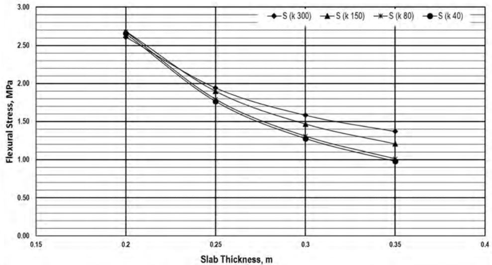
Stress Chart for Bottom-up Cracking Analysis Without Concrete Shoulders ( P=80\text{ kN} , \Delta T=15^\circ\text{C} )
