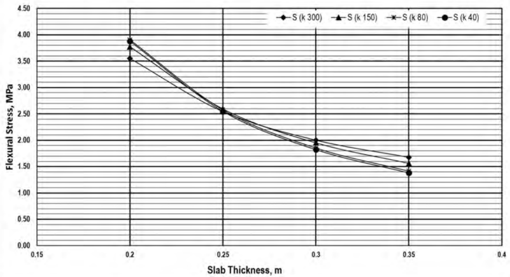
Stress Chart for Bottom-up Cracking Analysis Without Concrete Shoulders ( P=120\text{ kN} , \Delta T=15^\circ\text{C} )
