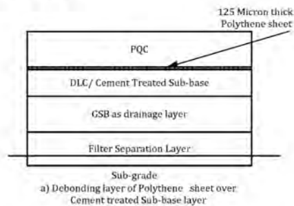
Figure 1 Typical Cross Section of Concrete Pavement -1
