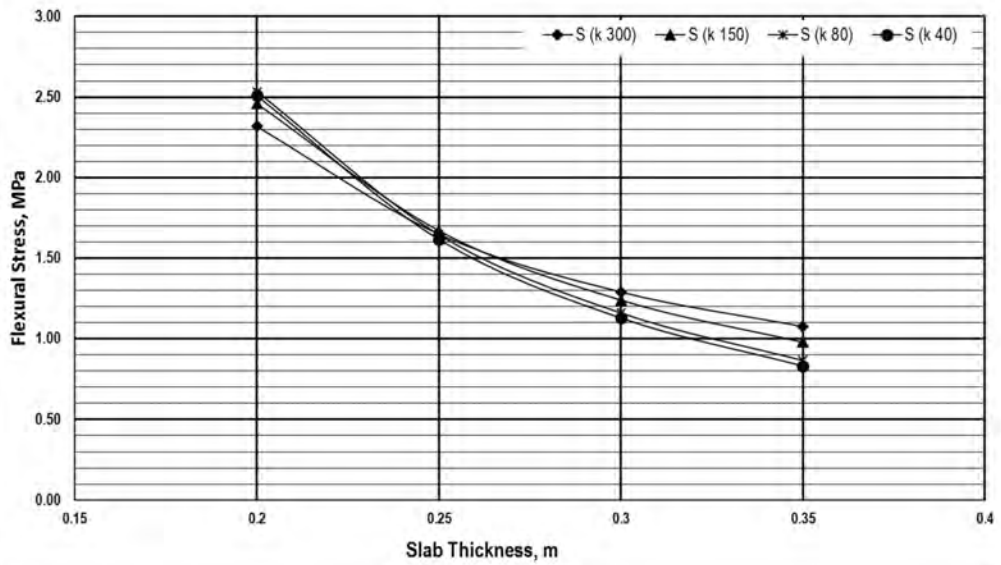
Stress Chart for Bottom-up Cracking Analysis Without Concrete Shoulders ( P=80\text{ kN} , \Delta T=10^\circ\text{C} )
