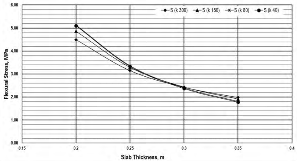
Stress Chart for Bottom-up Cracking Analysis Without Concrete Shoulders ( P=160\text{ kN} , \Delta T=15^\circ\text{C} )
