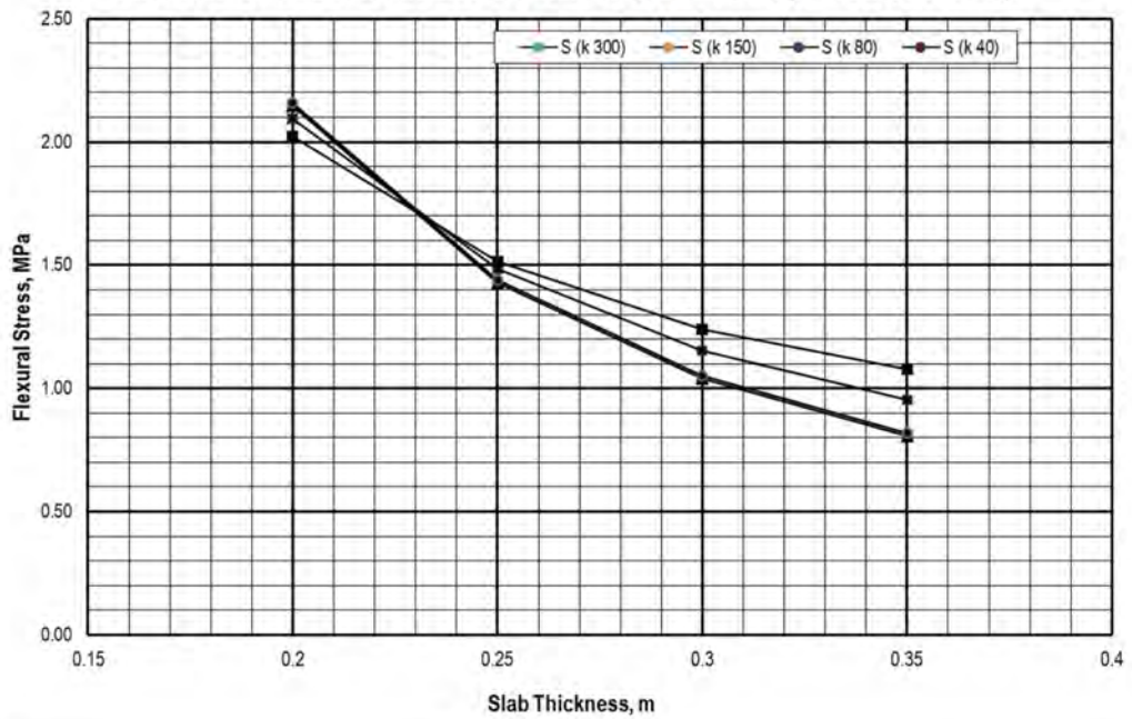
Stress Chart due to Tandem Axle Load with Concrete Shoulder ( P=200 kN, \Delta T=15^\circ C)
