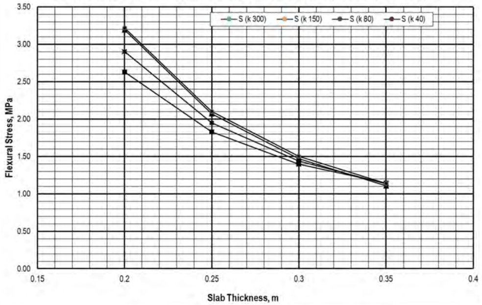
Stress Chart due to Tandem Axle: without Concrete Shoulder ( P=240 \text{ kN} , \Delta T=10^\circ\text{C} )
