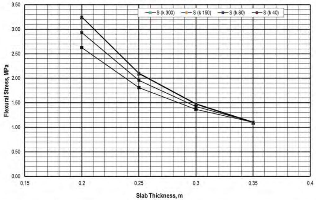
Stress Chart due to Tandem Axle Load with Concrete Shoulder ( P=320 \text{ kN} , \Delta T=10^\circ \text{ C} )
