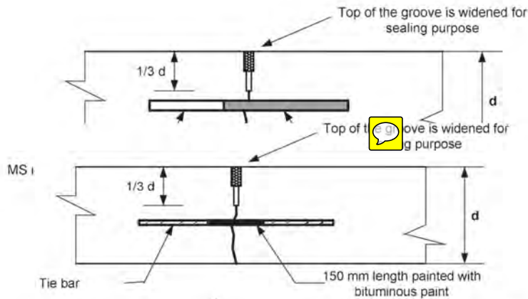
Figure 12 Longitudinal joint with tie rod between two lanes
