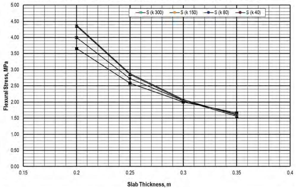
Stress Chart due to Tandem Axle: without Concrete Shoulder ( P=320 \text{ kN} , \Delta T= 15^\circ\text{C} )
