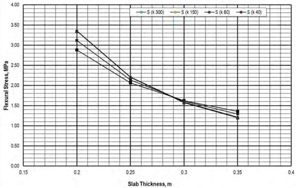
Stress Chart due to Tandem Axle Load with Concrete Shoulder ( P=320 \text{ kN} , \Delta T=15^\circ \text{ C} )
