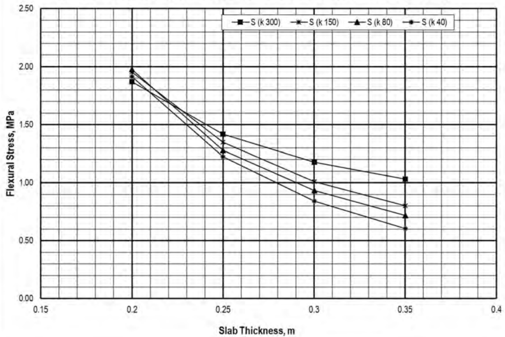
Stress Chart due to Single Axle Load with Concrete Shoulder ( P=80 \text{ kN} , \Delta T=10^\circ \text{C} )
