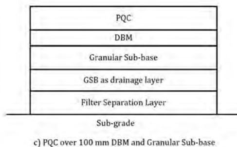
Figure 3 Typical Cross Section of Concrete Pavement -3
