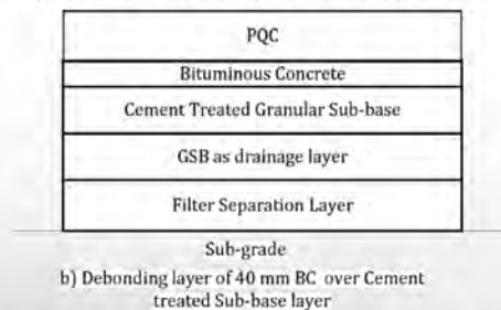
Figure 2 Typical Cross Section of Concrete Pavement -2
