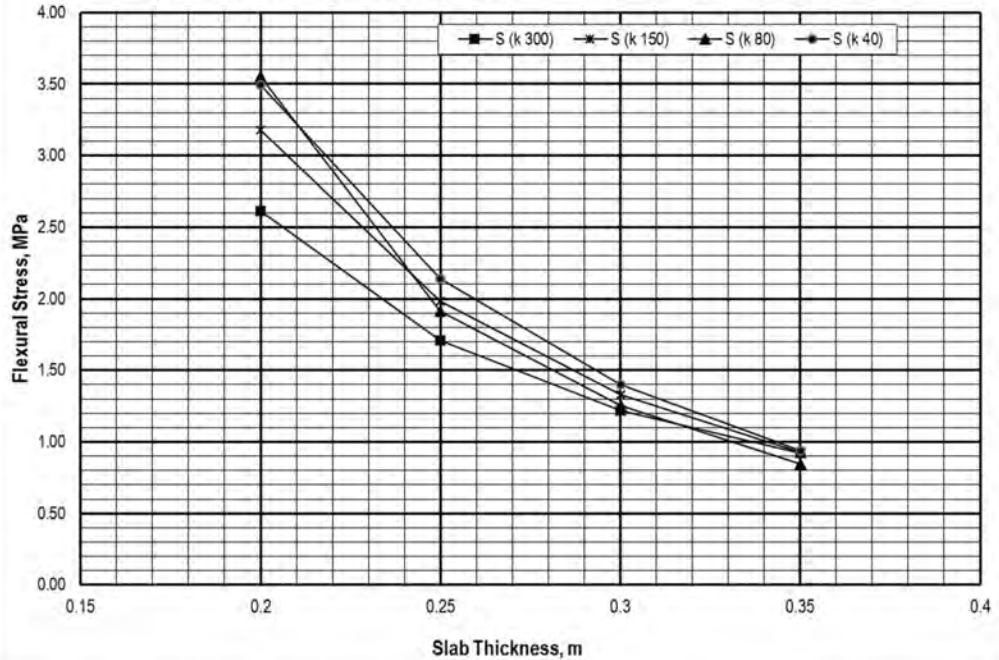
Stress Chart due to Single Axle Load with Concrete Shoulder ( P=160 \text{ kN} , \Delta T=0^\circ \text{C} )
