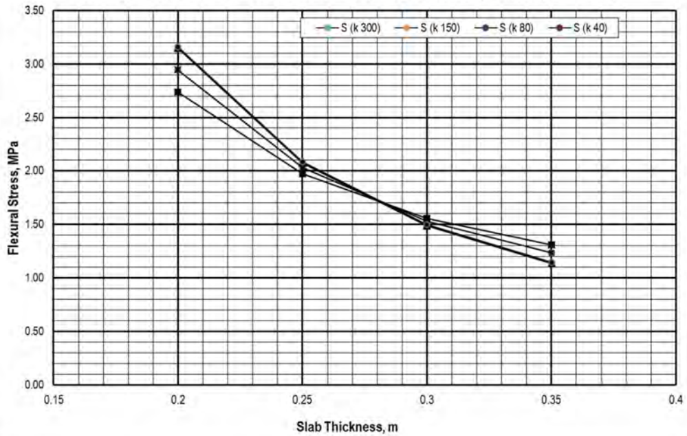
Stress Chart due to Tandem Axle Load with Concrete Shoulder ( P=300 \text{ kN} , \Delta T=15^\circ \text{ C} )
