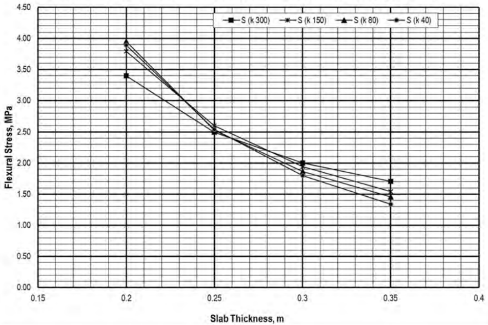
Stress Chart due to Single Axle Load with Concrete Shoulder ( P=160 \text{ kN} , \Delta T=15^\circ \text{ C} )
