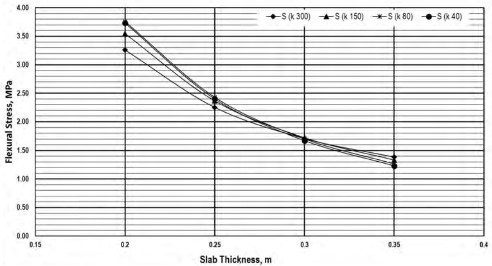
Stress Chart for Bottom-up Cracking Analysis Without Concrete Shoulders ( P=120\text{ kN} , \Delta T=10^\circ\text{C} )
