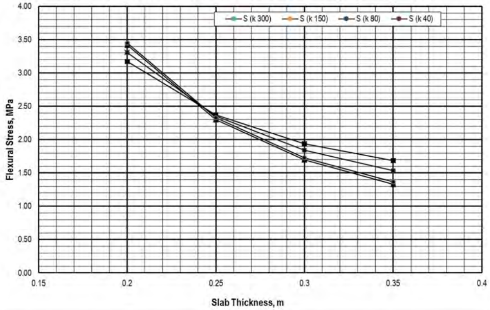
Stress Chart due to Tandem Axle: without Concrete Shoulder ( P=240 \text{ kN} , \Delta T=20^\circ\text{C} )
