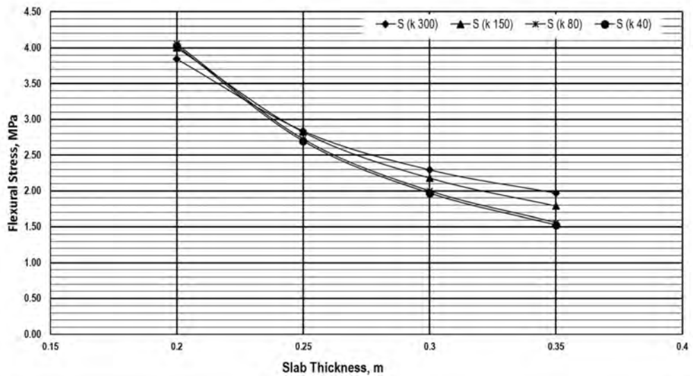
Stress Chart for Bottom-up Cracking Analysis Without Concrete Shoulders ( P=120\text{ kN} , \Delta T=20^\circ\text{C} )
