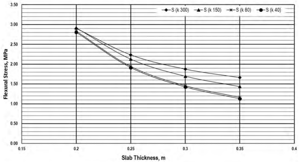
Stress Chart for Bottom-up Cracking Analysis Without Concrete Shoulders ( P=80\text{ kN} , \Delta T=20^\circ\text{C} )
