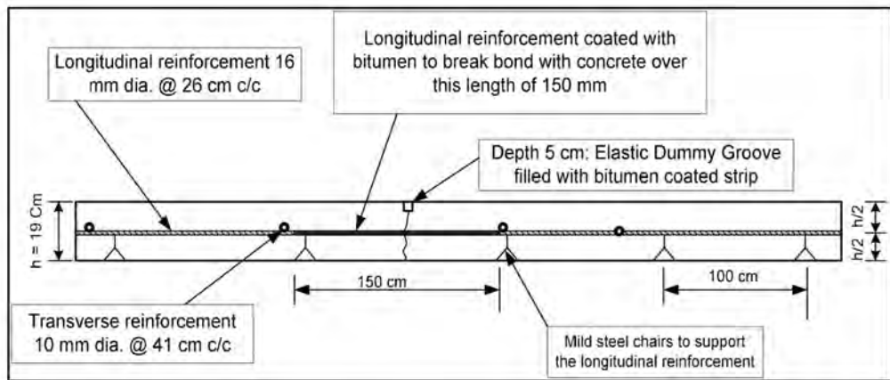
Figure 144 Details of Elastic Joint Section
